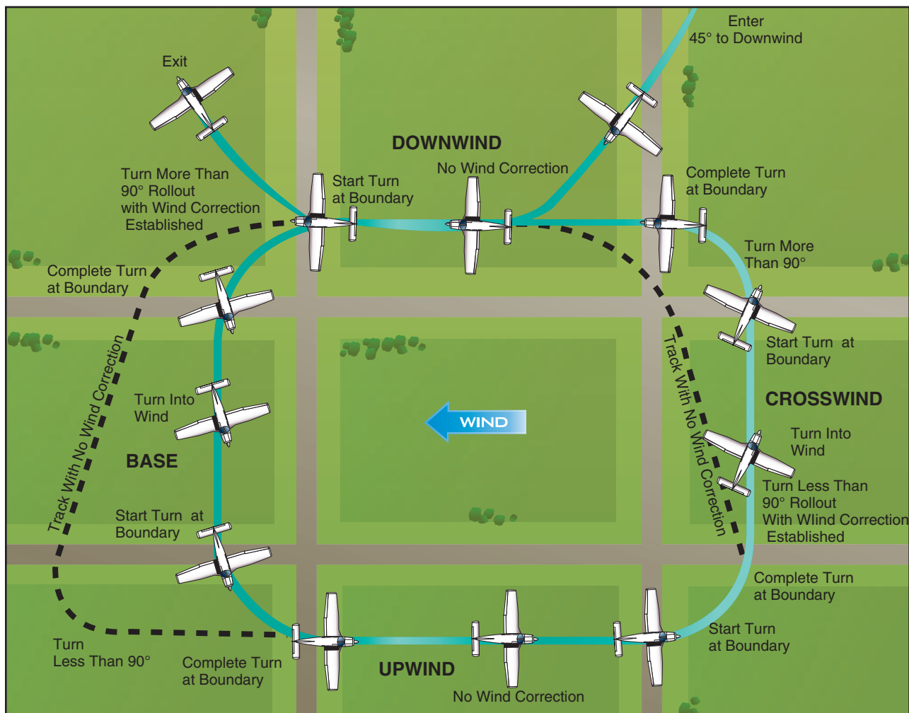
Figure 6-4. Rectangular course.
